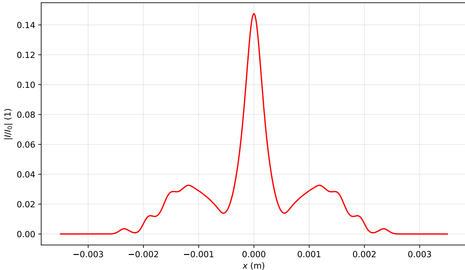
Intensity profile I(x, y = 0, z = 3.344)/I_0 , P_{in}=8.5P_{cr} , artificial time
